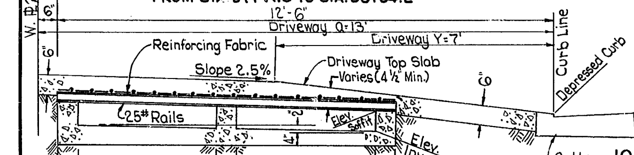
SECTION J-J FROM STA. 98+77.25 TO STA. 99+00.75
