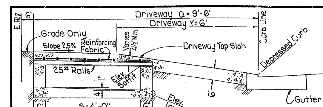
SECTION F-F FROM STA. 99+39 TO STA. 99+72
